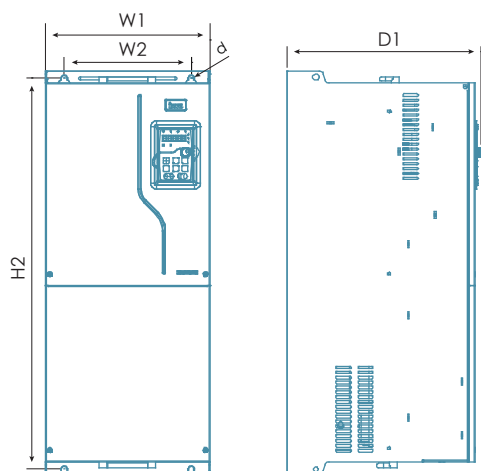
AC 3PH 380V 160~200kW mounting diagram
