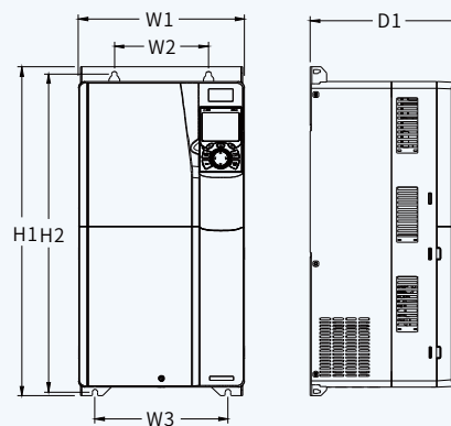
Outline and mounting dimensions for E9 frame
