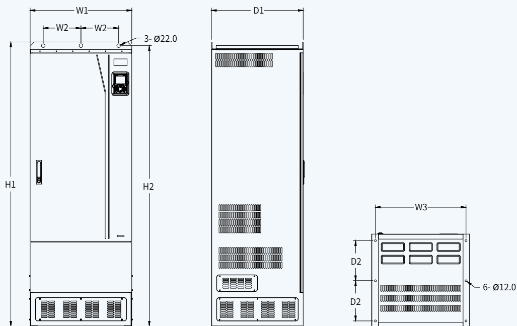
Outline and mounting dimensions for E14 frame
